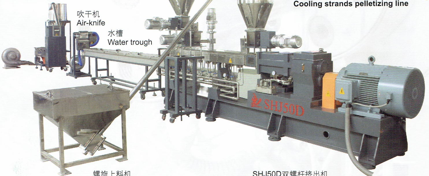
螺旋上料机 Spiral solids conveyer
